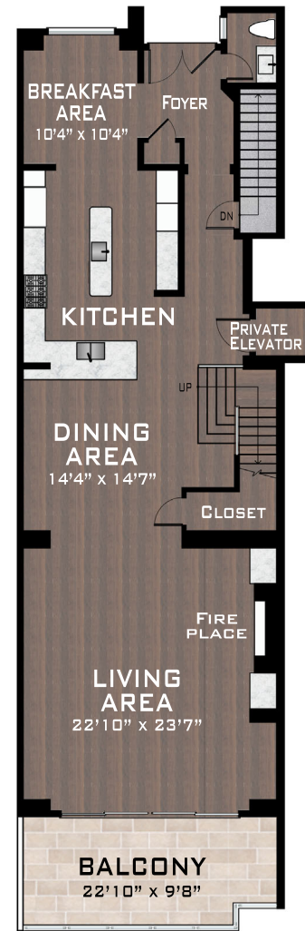
FIRST FLOOR
