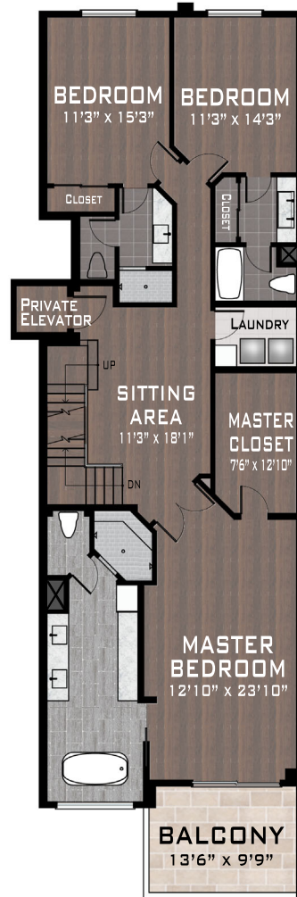
SECOND FLOOR
